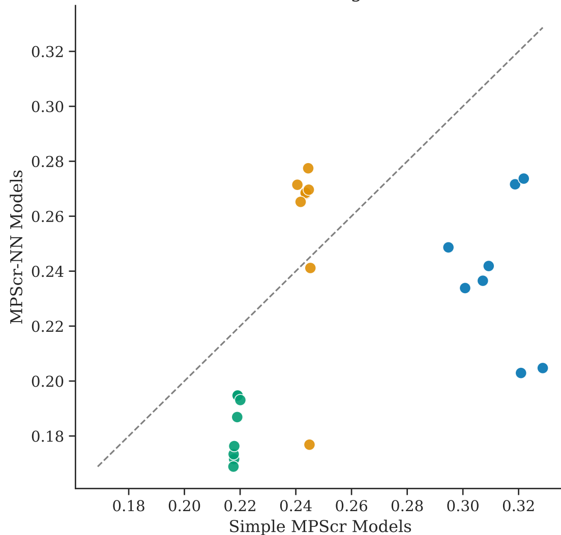
Anderson-Darling Statistic
