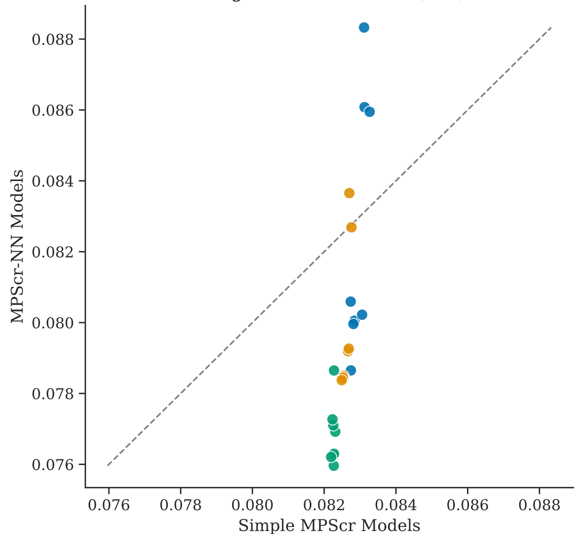
Integrated Brier Score (IBS)
